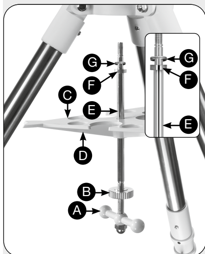
Fig. 4 Fastening of spreader plate and spacer ring
