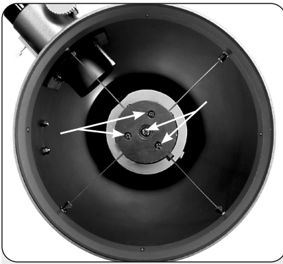
Fig. 31b: The four collimation screws in the secondary mirror housing
